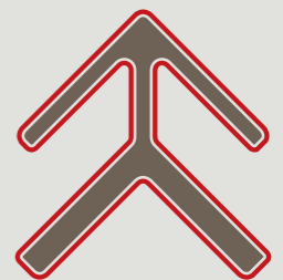
Outside Corner Trim US46 55 x 59 mm (2.2 x 2.3 in)
